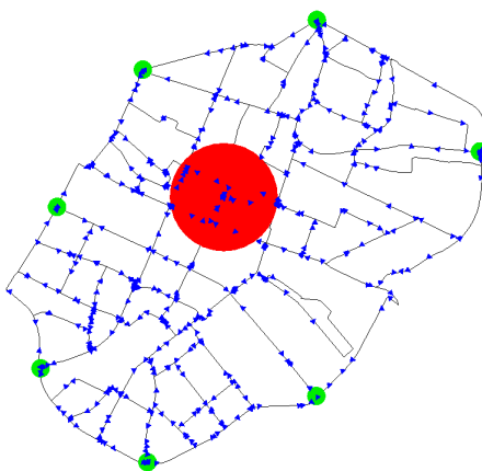
Figure 6. Snapshot of the city evacuation model: the red circle is the hazard perception area, the green circles the evacuation sites and the blue triangles the drivers.
