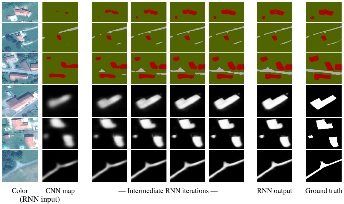
Figure 5: Evolution of fragments of classification maps (top rows) and single-class fuzzy scores (bottom rows) through RNN iterations.
