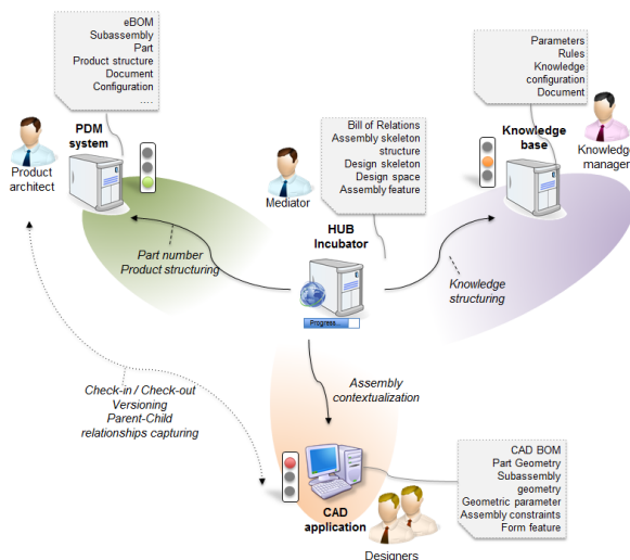
Fig. 1. Incubator concept.
