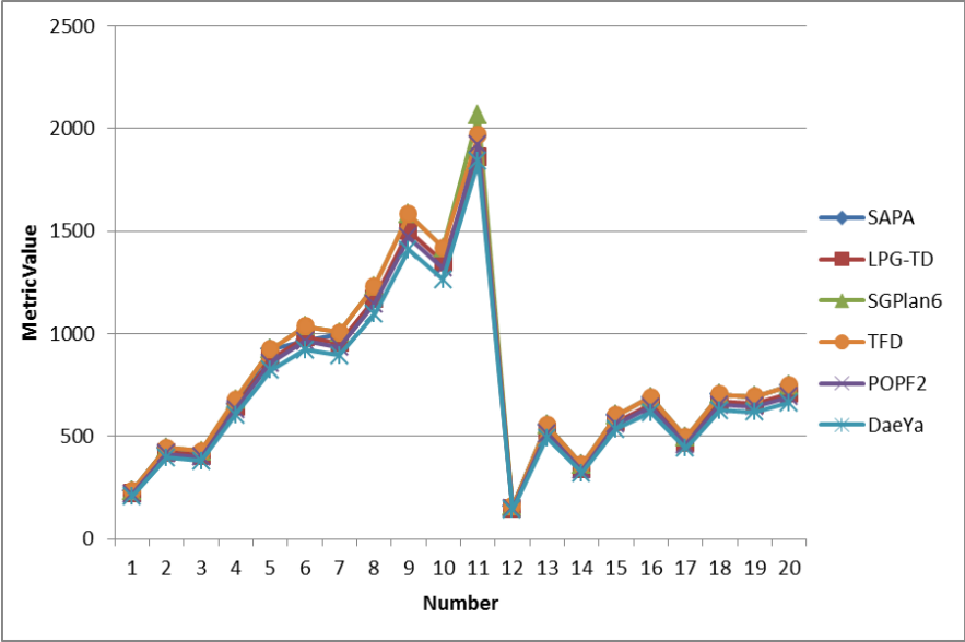
Fig. 1. DVRP Benchmark
