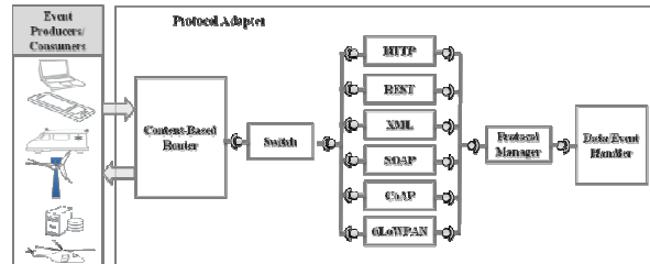
Fig. 7: Protocol Adapter Architecture
