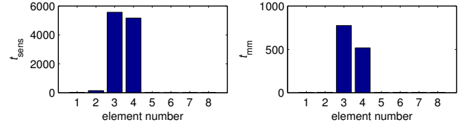
Figure 4: Sensitivity (left) and minmax tests (right) for 5% damage in element 3 and 10% damage in element 4.
