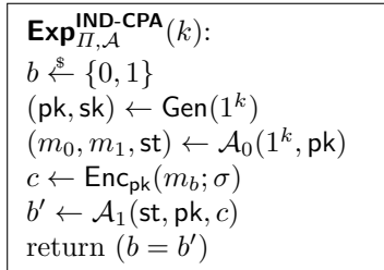
Fig. 1. IND-CPA experiment.
