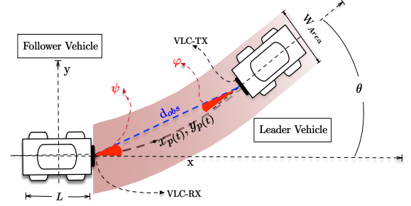
Fig. 3. Laser based preceding vehicle detection and VLC for two platoon members. L represent the vehicle length and W_{Area} is width of the laser detection area of interest. \psi and \phi are VLC incidence and irradiance angles.
