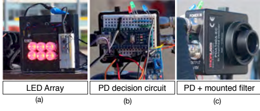
Fig. 5. VLC transmitter and receiver ends.
