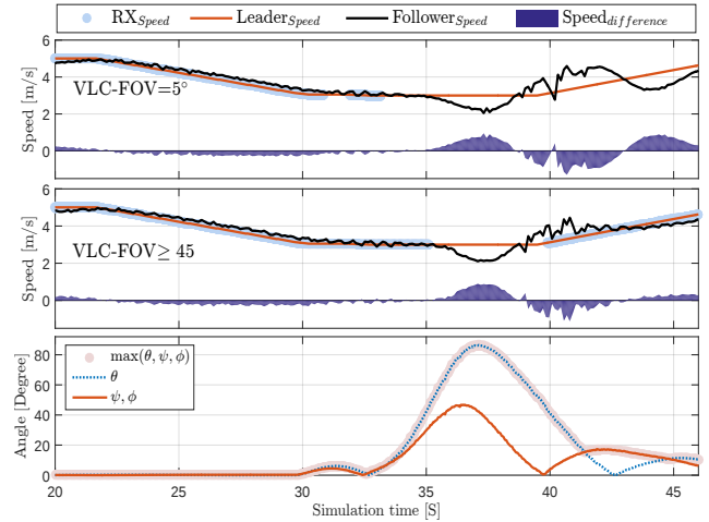
Fig. 11. Simulation results of Curve driving platoon scenario.
