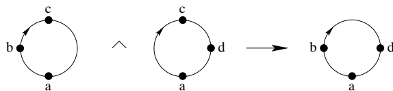
Fig. 2. Ternary Transitivity
