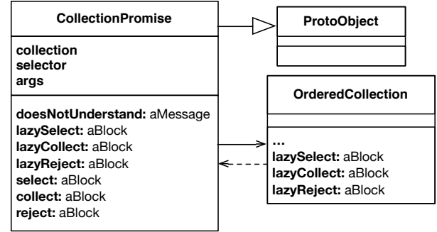
Figure 2. Implementation - Class Diagram
