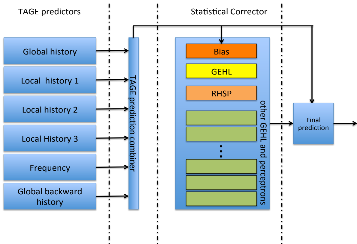
Figure 1: Prediction computation flow on the MTAGE-SC predictor
