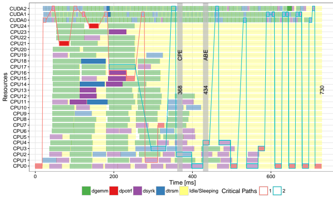
Fig. 5: Detailed view (see http://perf-ev-runtime.gforge.inria.fr/vpa2016/ ) of a 12 \times 12 Cholesky execution (DMDAS scheduler) with two (red and blue) critical paths.
