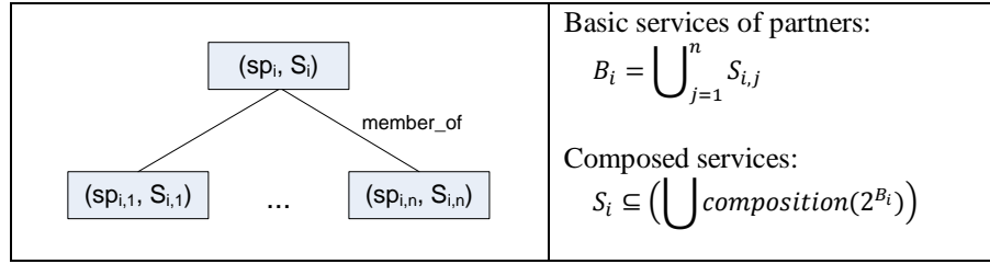
Fig. 13. A service provider as a composition of other service providers
