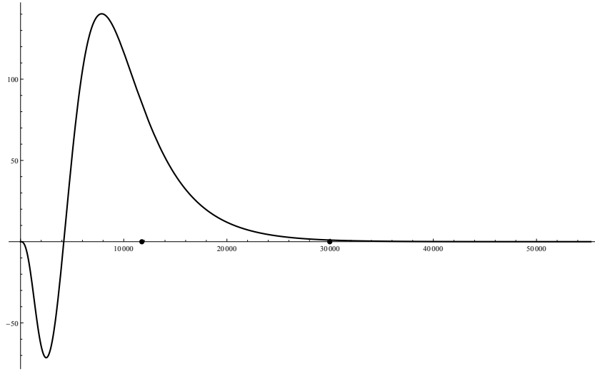
Fig. 2: Graphs of the difference \mathbf{E}[S_4(t)] - \mathbf{E}[P_4(t)] for n = 1000 . S_4(t) is the number of black balls in the serial model and P_4(t) is the number of black balls in the parallel model.
