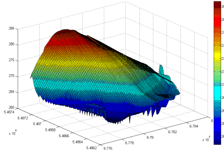
Fig.6. Three-dimensional topographic surface map
