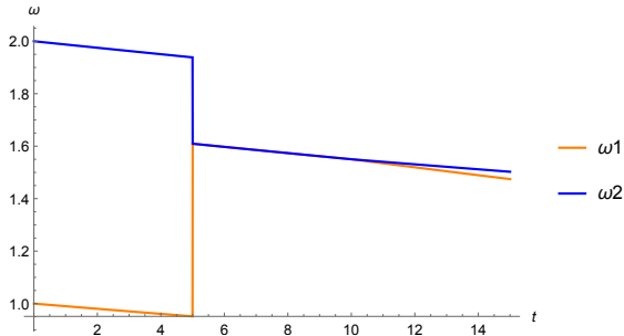
Figure 1: Simulation of the clutch model with resets. Mode change F → T occurs at t = 5 s and mode change T → F occurs at t = 10 s.
