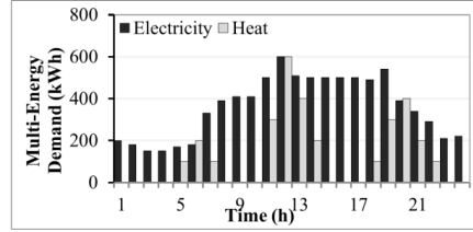
Fig.2. Electricity and heat consumption of MED.
