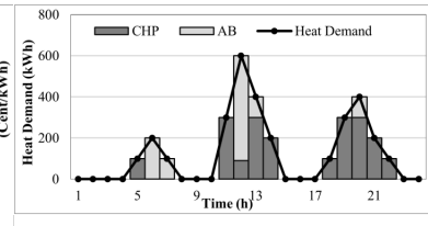
Fig.5. Heat operation scheduling of micro-MES in Case I.
