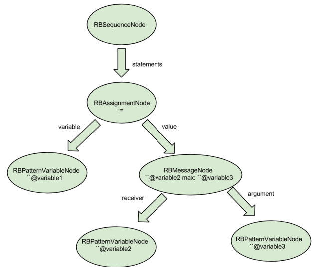
Figure 4. AST representation of listing 7 snippet (RHS)
