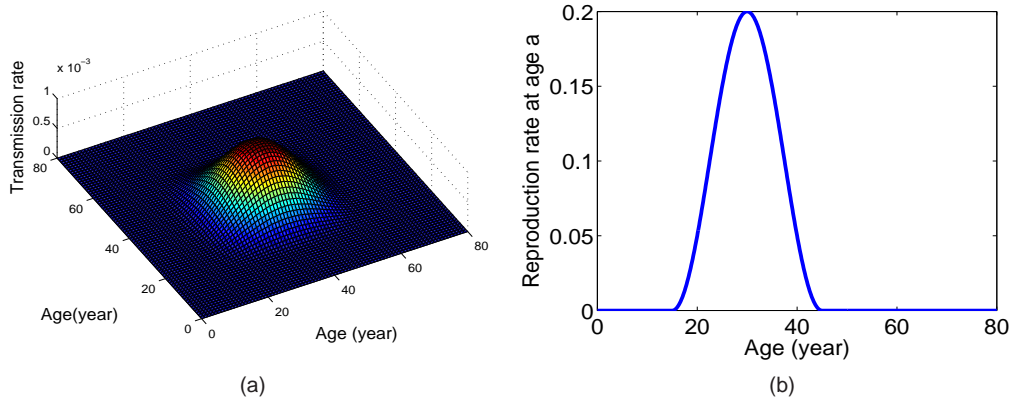
Figure 1: (1a) Transmission coefficient \beta(.,.) when the transmission constant \beta_0 = 10^{-3} . (1b) Fecundity function f(.) .
