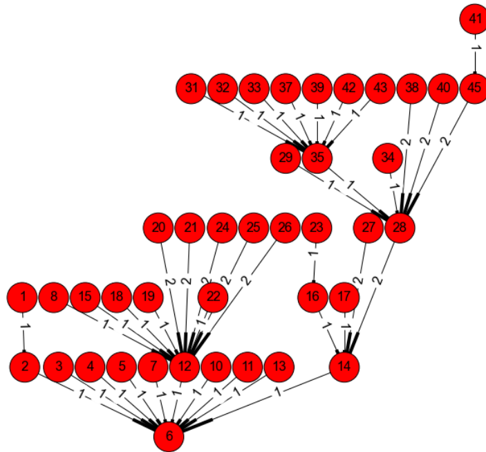
Figure 8: Example of a distance tree computed by nodes.
