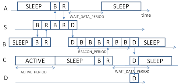
Figure 2: Illustrative diagram for data routing in ODYSSE.
