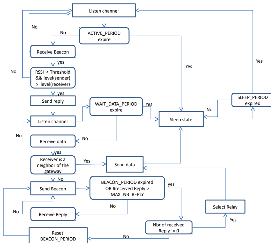
Figure 23: The flowchart of router nodes in ODYSSE.
