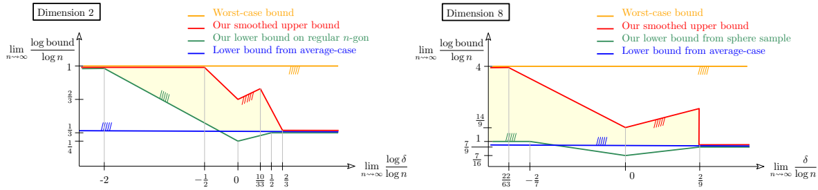
(a) A comparison of our smoothed complexity bound for Euclidean perturbation (Theorem 5 and Corollary 6) and two lower bounds, where the initial points are placed respectively at the vertices of a unit-size n -gon (Theorem 7) and in the origin. A data point with coordinates (x, y) means that for a perturbation with \delta of magnitude n^x the expected size of the convex hull grows as n^y , subpolynomial terms being ignored. The worst-case bound is given as a reference. The constants in the O() and \Omega() have been ignored as their influence vanishes as n \rightarrow \infty in this coordinate system.
