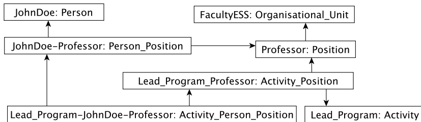
Fig. 4. An excerpt of the activity model describing University activities, roles and responsibilities
