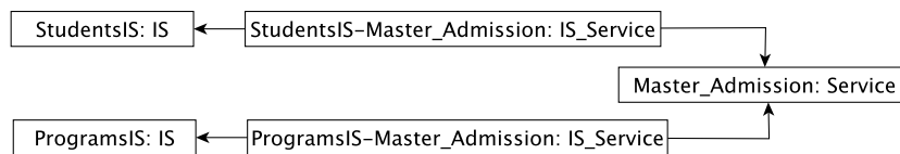
Fig. 12. An excerpt of service model representing a service built on two IS
