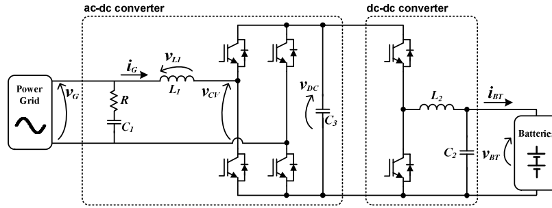
Fig. 2. On-board bidirectional battery charger composed by two power converters: ac-dc full-bridge bidirectional converter and dc-dc buck-boost bidirectional converter.
