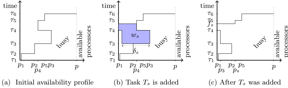
Figure 3: Processor availability behavior with GREEDYFILLING.
