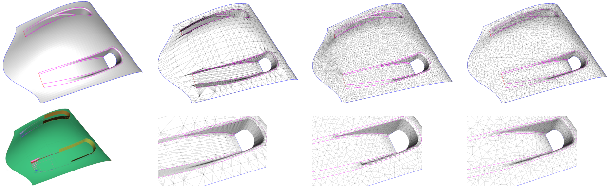
Figure 11: Scoop . Top: NURBS model with sharp edges depicted in pink, smooth edges in red, open boundary in blue; mesh (7k triangles) generated by Rhino, GMSH and our approach ( \epsilon = 0.001 ). Bottom: NURBS surfaces, closeups on above meshes.
