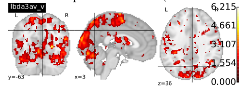
(b) Multivariate Hurst exponent estimation ( \lambda = 3 ).
