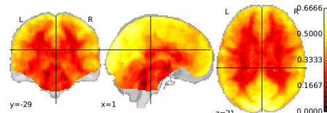
Fig. 2. Median value of Hurst exponents estimated on real rs-fMRI data from the 36 individuals using the univariate wavelet-based estimator.
