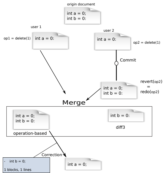
Figure 11. undo/redo operation
