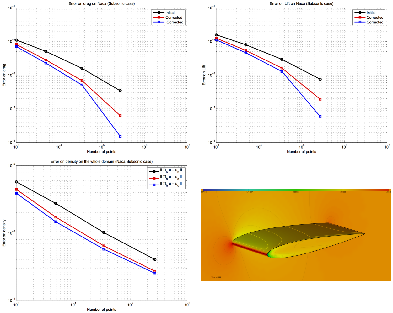
Figure 4. 3D Naca subsonic case: Error on drag (top left), error on lift (top right), implicit error in L^2 norm on the density without and with corrections (bottom left), and density iso-values on the wing (bottom right). Plain black line is the uncorrected solution while plain red lines is the corrected solution (I) based on \mathcal{F}_{\frac{h}{2}}(W_h) and plain blue line is the corrected solution (II) with \mathcal{F}_{\frac{h}{2}}(R_h W_h) .
