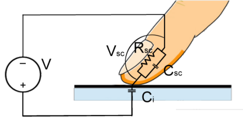
Fig. 3. Electrical representation of the stratum corneum
