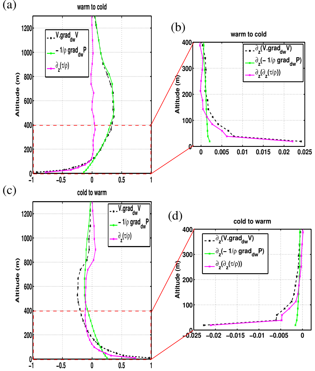
Fig. 11: Composite terms of the downwind momentum balance anomaly above downwind SST gradient anomalies with intensity larger than 2.10^{-5} \text{ }^{\circ}\text{C m}^{-1} . Balance is for July 2007 in CPLM over the Peru region. (a) Composite terms above negative downwind gradient anomalies (warm to cold transition). Downwind momentum balance anomalies (eq. (10)) terms are: Lagrangian acceleration of the air parcel along the streamline (black), momentum turbulent mixing (magenta), pressure term (green), units are 10^5 \text{ m}^2 \text{ s}^{-2} \text{ }^{\circ}\text{C}^{-1} . Terms have been normalized by the downwind gradient anomalies intensity. (b) vertical shear of the profiles shown in (a), in 10^5 \text{ m s}^{-2} \text{ }^{\circ}\text{C}^{-1} . (c) same as (a) but for positive downwind gradient anomalies (cold to warm transition). (d) vertical shear of the profile shown in (b)
