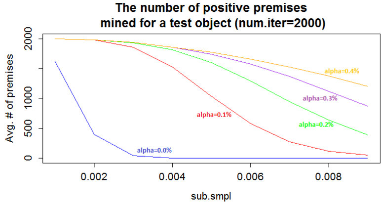
Fig. 2. The dynamics of \alpha - weak positive premises mining
