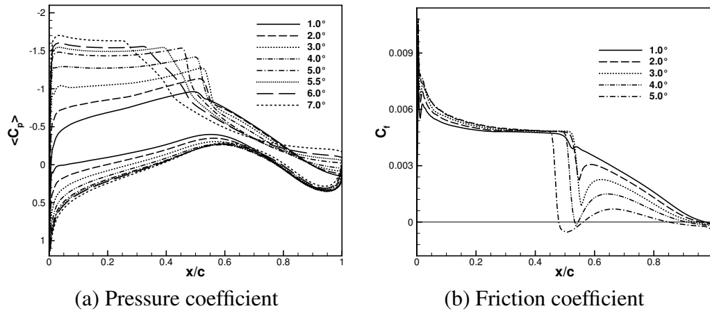
Figure 2: Effect of the angle of attack on the steady and mean surface distributions and on the friction coefficient
