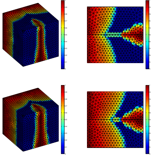
Figure 6: A single vertical fracture: saturation of the injected wetting fluid at two different times. At left saturation on \partial\Omega . At right saturation on the bottom face of \Omega .
