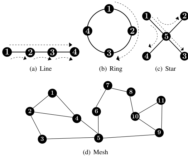
Fig. 4. Considered network topologies.
