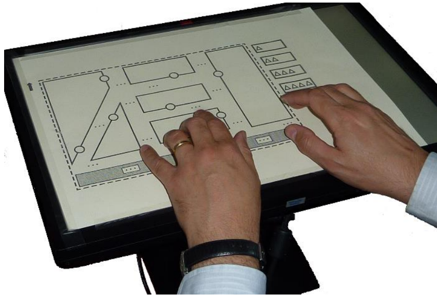
Figure 3: Interactive audio-tactile map prototype composed of a multi-touch screen with raised-line overlay
