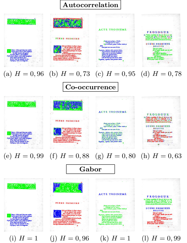
Figure 3: Result examples of texture feature evaluation on simplified historical document images. For the same page, each cluster (represented by a given color) represents a similar or homogeneous region. Because the process is unsupervised, the color attributed to text or graphics may differ from one document image to another.
