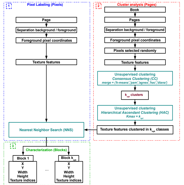
Figure 1: Presentation of our pixel labeling approach for historical digitized book content.
