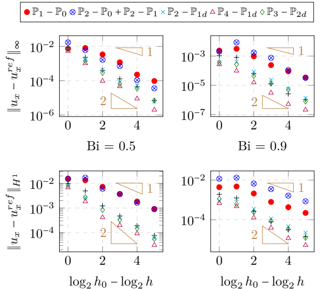
Figure 5: L_\infty -norm (top) and H^1 -norm (bottom) convergence plots for various FEM approximation orders, for Bi = 0.5 (left) and Bi = 0.9 (right). u_x^{ref} denotes the analytic solution.
