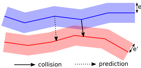
Figure 5: Example of an accepted and predictive ray in a cloth \rightarrow cloth test. The ray is accepted if its length is inferior to e + e' .
