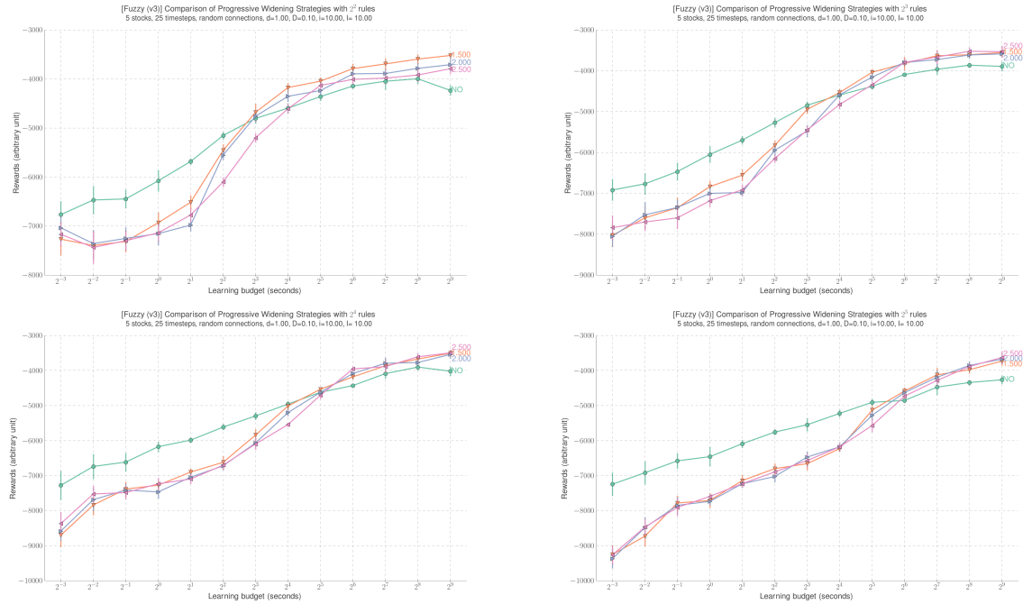
Fig. 7. Case of Eq. 1, smaller test case, logarithmic Sieves. “NO” stands for the default version, with no Sieves method. Triangles correspond to Sieves methods, with rate given in the legend. We compare our Sieves method to cases in which we restrict a priori the number of rules to 1, 2, 4, 8, 16 rules. More precisely, in each case, there is the default method (fixed number of rules) and our method (variable number of rules, reaching the same number for the largest budget). Basically, the Sieves method always works.
