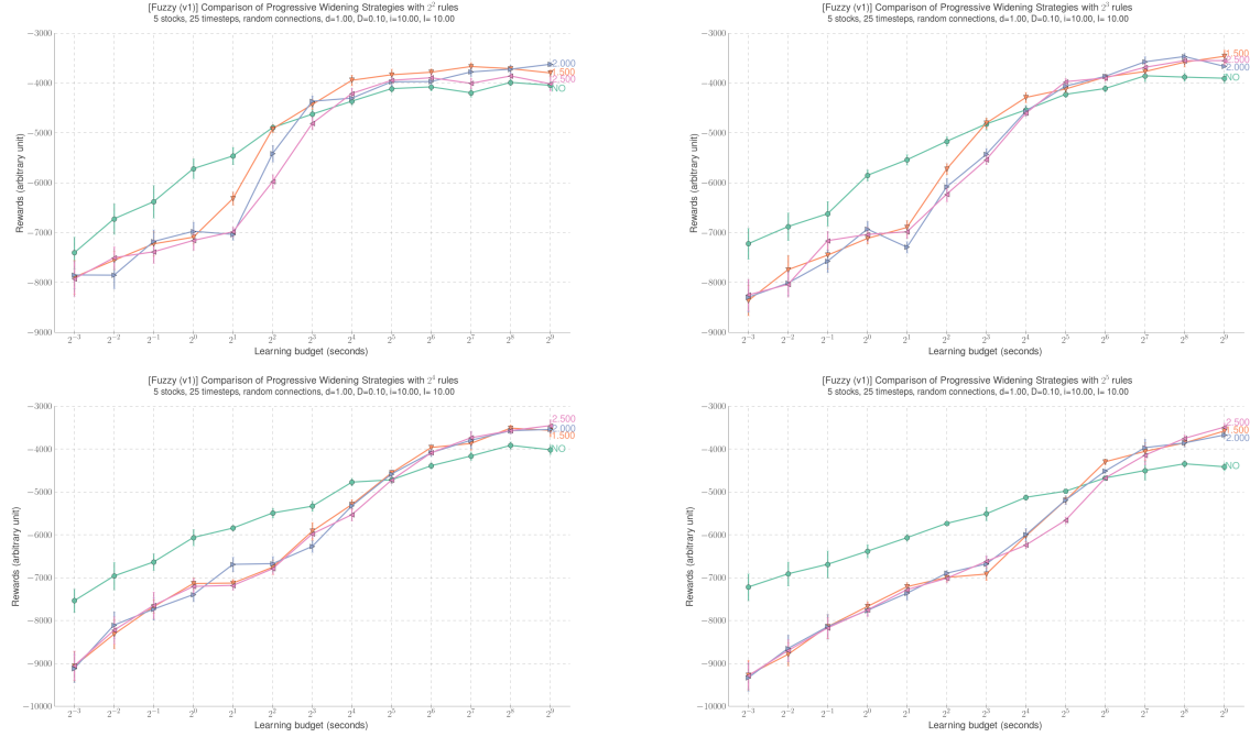
Fig. 6. Results with Eq. 4, smaller test case, and the smaller test case, logarithmic Sieves. “NO”: no Sieves method. Triangles correspond to Sieves methods with various rates, in the case of a linear rate. We compare our Sieves method to cases in which we restrict a priori the number of rules to 1, 2, 4, 8, 16 rules. More precisely, in each case, there is the default method (fixed number of rules) and our method (variable number of rules, reaching the same number for the largest budget). Basically, the Sieves method always works asymptotically.
