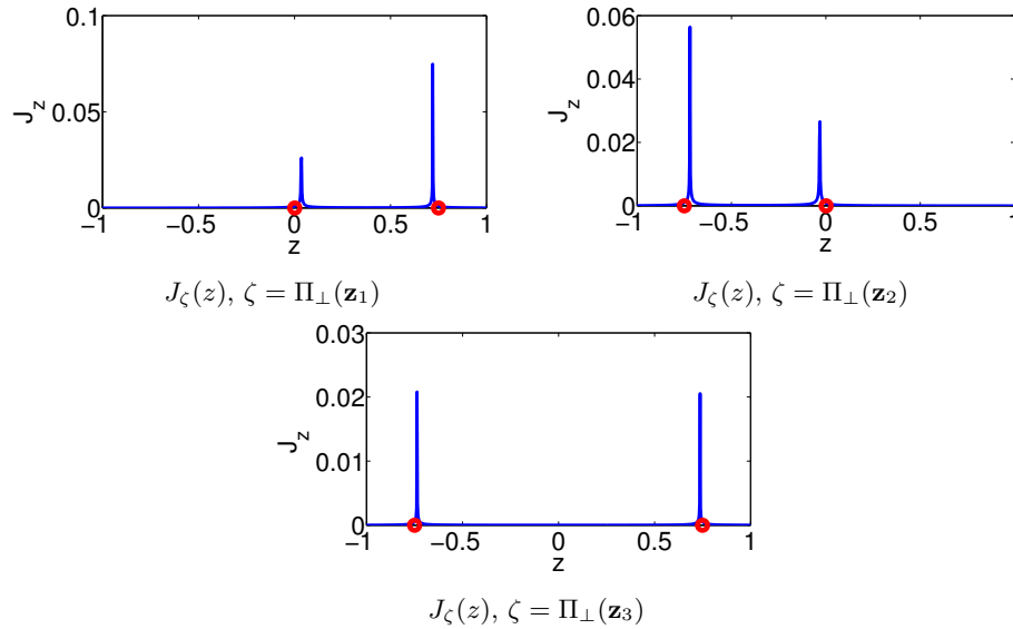
Figure 12: When J_{\Pi_\perp(\mathbf{z}_j)} is computed, peaks appear for i \neq j . Red circles show exact location of L(\mathbf{z}_j) .
