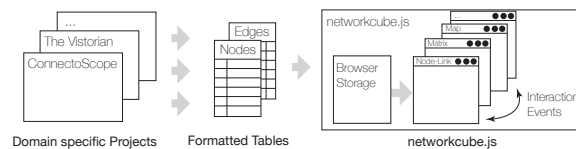
Figure 3: NetworkCube pipeline
