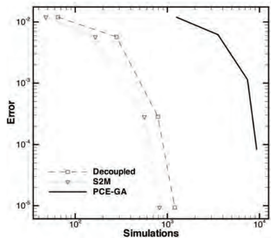
Convergence rates of the S2M method with respect to other classical techniques for robust design optimization (short column test function)
