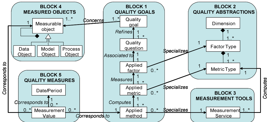
Figure 2 - Quality assessment meta-model
