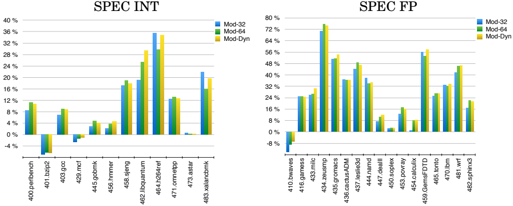
Fig. 7. IPC gain over the baseline for a clustered RBWiiffccw configuration with an inter-cluster delay of 3 cycles: benchmark per benchmark comparison of Mod-32 steering, Mod-64 and adaptive Mod-N.
