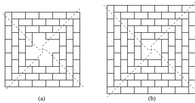
Fig. 4: Graphs of non-fixed edges for (a) \mathcal{A}_{QT}(12, bbbaaa) (b) \mathcal{A}_{QT}(14, bbcaaaa)
