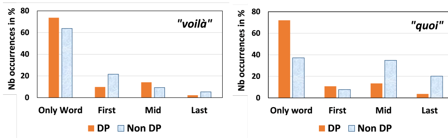
Fig. 2. Position of voilà and quoi in the intonation groups
