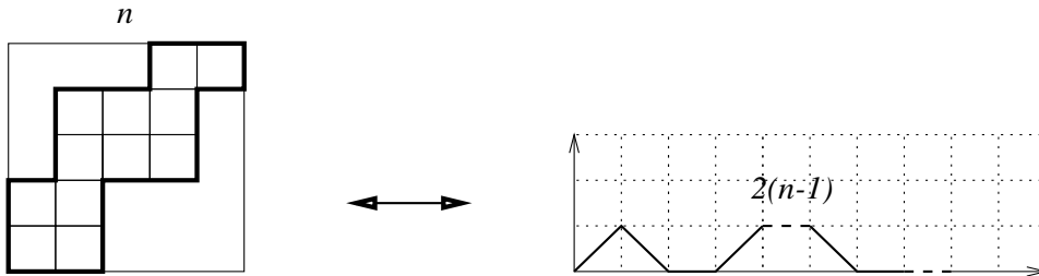
Fig. 14: A particular case of the bijection is the restriction to parallelogram polyominoes and positive cycles.
