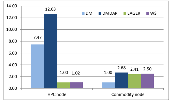
Figure 8: Impact of the scheduling algorithms for experiments on heterogeneous platforms. Relative speedup over the worst situation on each platform.
