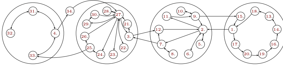
Fig. 54: Overview of the proofs.
