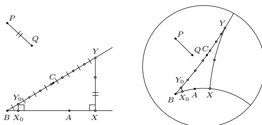
Fig. 53: Axiom 2 implies Axiom 3.
