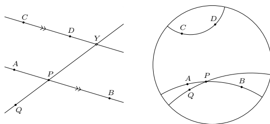
Fig. 31: Proclus' postulate (Postulate 13).
