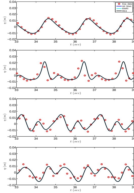
Figure 11: Time series of surface elevation, for the FV scheme, at wave gauges 4,5 (up) 8,10 (down) for periodic wave propagation over a bar
